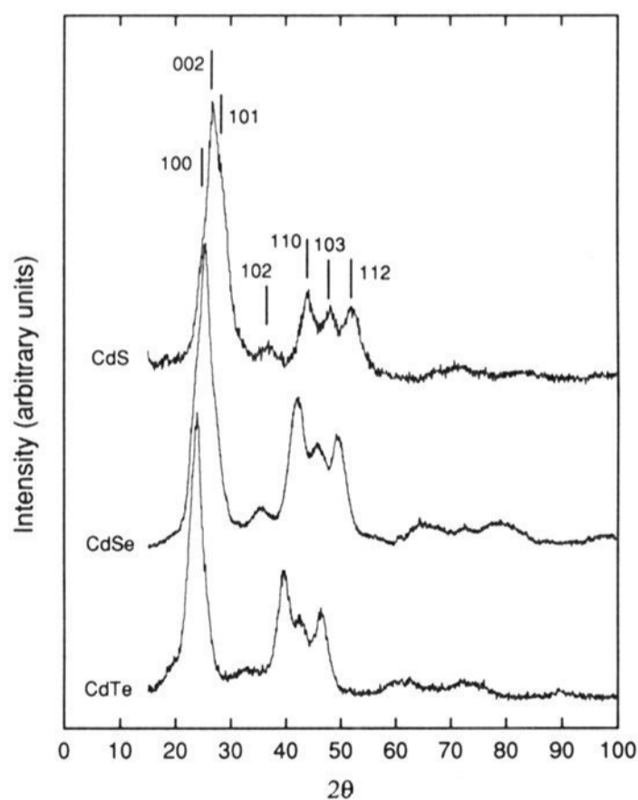
Figure 10. Powder X-ray diffraction spectra of \sim 35 Å CdS, CdSe, and CdTe crystallites. The positions of bulk reflections for wurtzite CdS are indicated.
