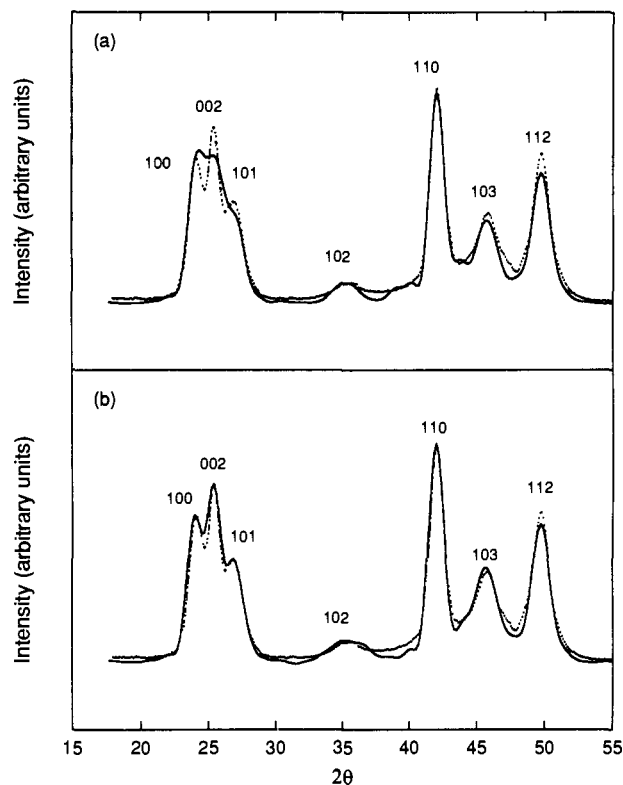
Figure 13. Experimental X-ray powder diffraction spectrum of ~80 Å diameter (~10 000 atoms) crystallites (dotted line) compared with computer simulations (solid line) of (a) spherical and (b) prolate particles [aspect ratio of 1.3 along the (002) direction]. Three stacking faults on average and bulk lattice constants are used.
