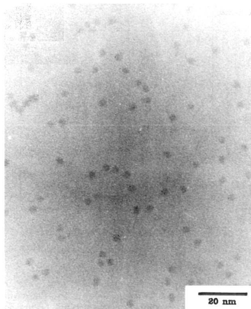
Figure 6. TEM image taken in bright field with lattice contrast shows a collection of slightly prolate particles. The elongated (002) axis measures 35.0 \text{ \AA} \pm 5\% while the perpendicular axis measures 30 \text{ \AA} \pm 6\% . The particles are well dispersed and not aggregated.
